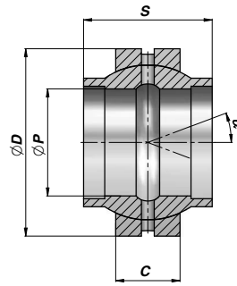
TYPE HHOH...2RS
